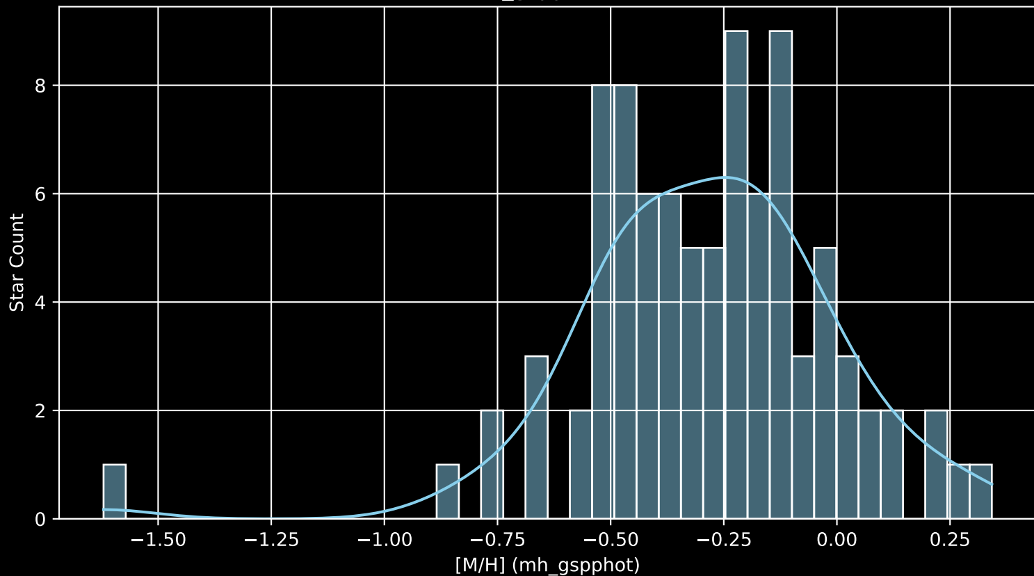
GALAH DR4 Field: [7154] [M/H] (mh_gspphot) (n= 90)
