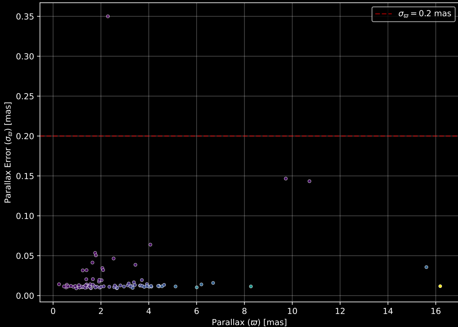
GALAH DR4 Field: [7154] Parallax Quality (n= 92)
