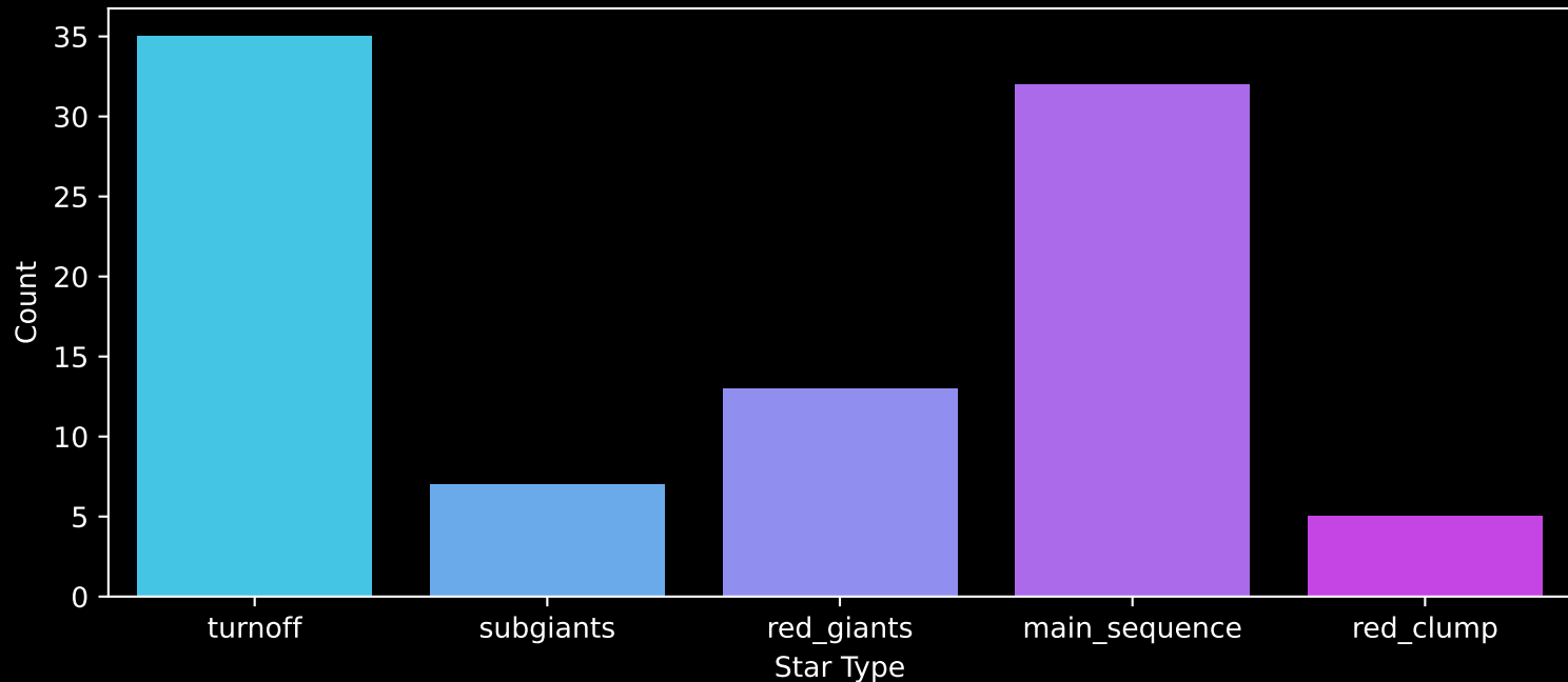
GALAH DR4 Field: [7154] Count plot of Star Type
