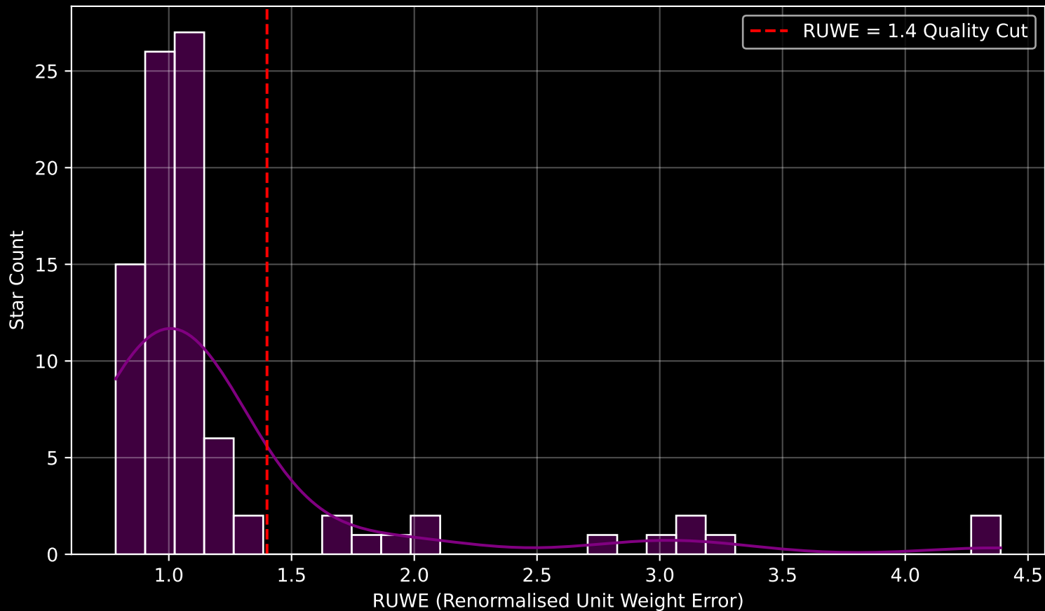
GALAH DR4 Field [7154] RUWE Distribution (n= 89)
