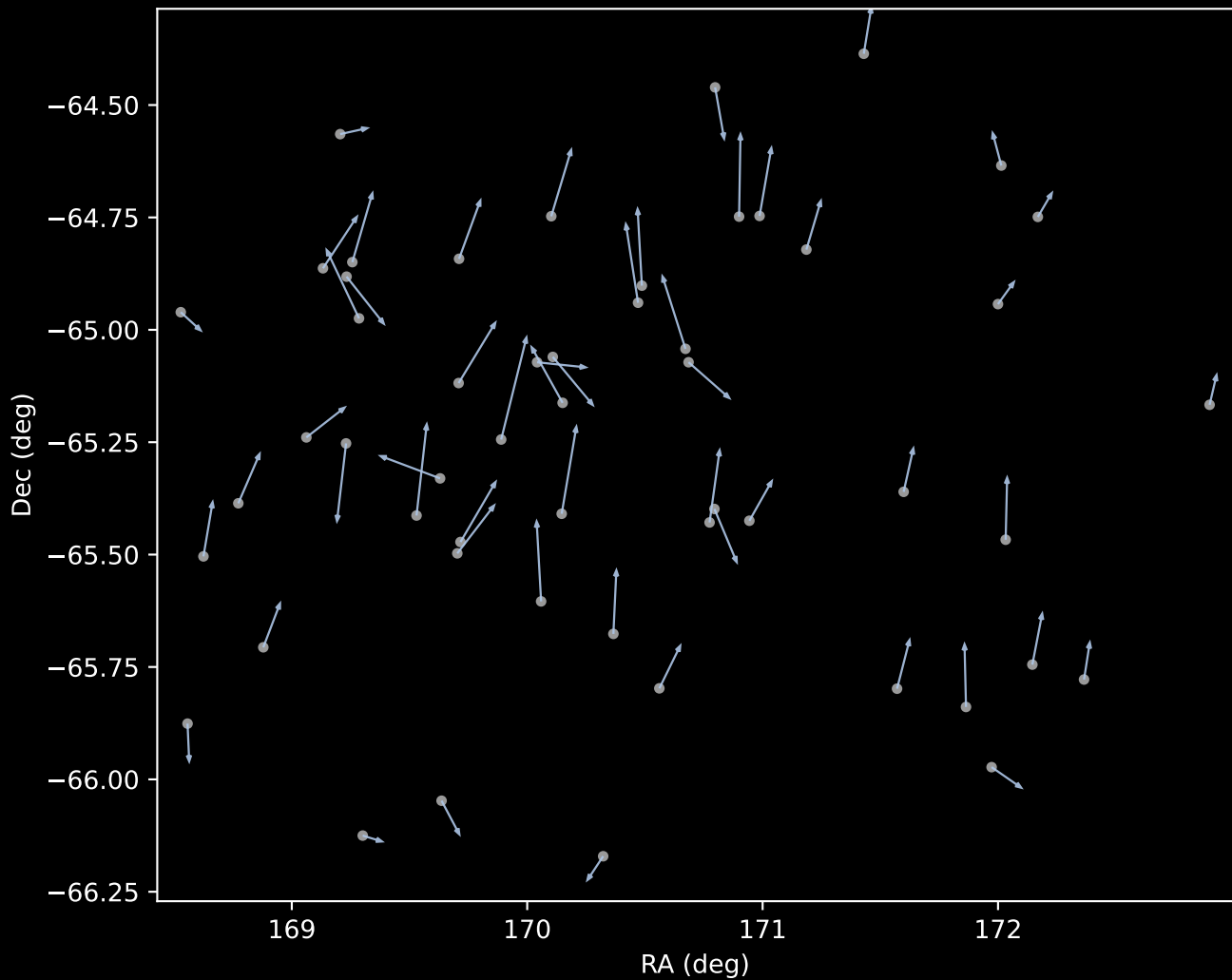
GALAH DR4 Cluster 1 Proper Motion Vectors (n=53)
