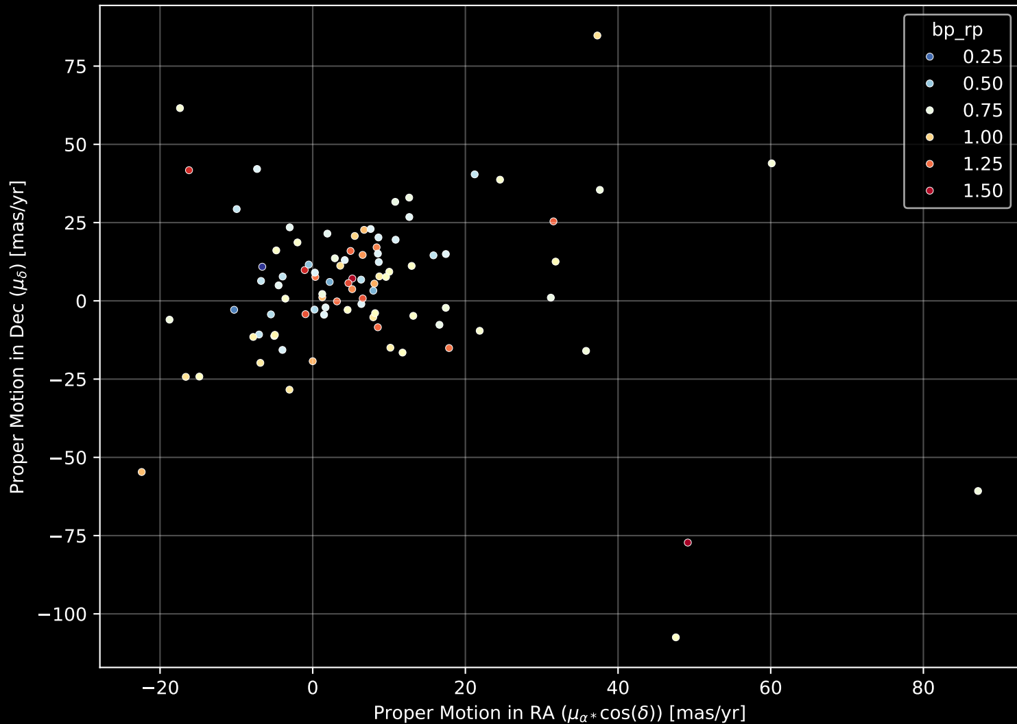
GALAH DR4 Field: [7154] Proper Motion Diagram (n= 92)
